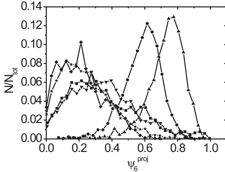
Figure 4-11 Distribution plot of the projected six-fold bond-orientational order parameter \psi_6^{proj} for the HCP-FCC transition. The different symbols correspond to a/a_{HS} = 1.055 (up-triangle), 0.986 (circle), 0.959 (down-triangle), 0.890 (diamond), 0.822 (star), and 0.753 (square).
