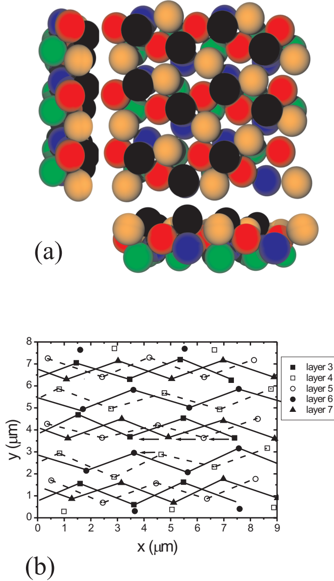
Figure 4-25 (a) Image showing particle coordinates in a small part of our real-space data-set in layers three to seven for the crystal at an anisotropically stretched template with a/a_{HS} = 1.076 and an axis ratio of c/c_{HS} \cdot (a/a_{HS})^{-1} = 1.50 . The image in the middle shows a top view, the other two the respective side views. Spheres, with diameter drawn to scale, have been colored corresponding to their layer-index: black for the top layer, then for subsequent layers respectively gold, red, blue and green. (b) A projection of xy particle coordinates for the spheres in (a) onto a single layer. The symbols corresponding to the different layers are given in the legend next to the graph. Positions indicated with filled symbols have been connected with solid lines, open symbols with dashed lines, in order to indicate the template-induced alignment. The arrows indicate the shift in particle positions with the original template ABA -sequence between layers 3, 5, 7, and 9 ( =3 ) and layers 4 and 6 respectively.
