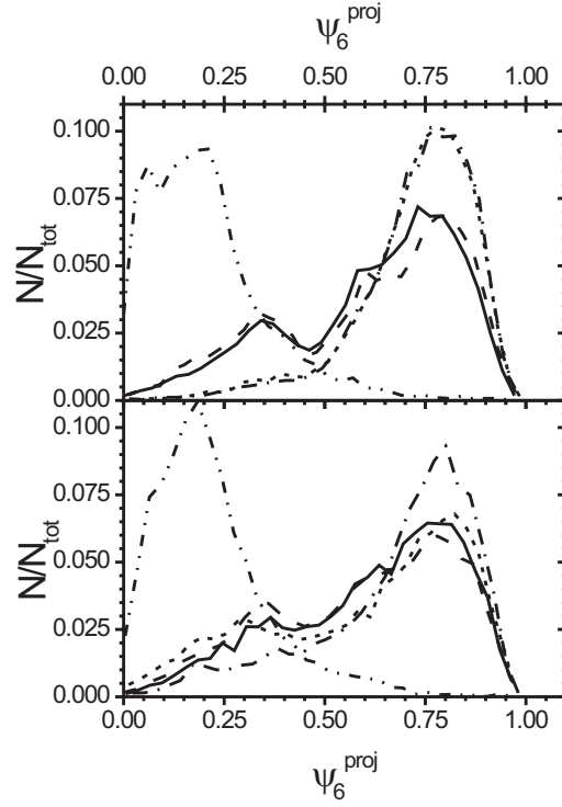
Figure 4-21 Distribution plots for \psi_6^{proj} for the anisotropically stretched template with a/a_{HS} = 1.076 for a projection of fourth and fifth layer (lower curves) and tenth and eleventh layer (upper curves). Different line types correspond to axis ratios of c/c_{HS} \cdot (a/a_{HS})^{-1} = 1.00 (solid line), 1.01 (dash), 1.02 (dash-dot), 1.07 (dash-dot-dot), and 1.50 (short dash) respectively.
