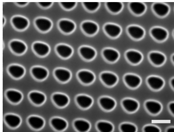
Figure 2-4 SEM image of a square-symmetric pattern of holes with a spacing of 140 nm in silicon. The PMMA-layer was written without switching the electron-beam off in between successive lattice positions. The scalebar indicates 100 nm.
