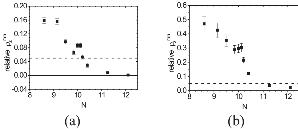
Figure 7-4 The evolution of the relative depth of the minimum in \rho_z for (a): the minimum in between the first and second layer, and (b): the minimum in between second and third layer. Note the change in scale on the vertical axis between (a) and (b). the dashed line indicates the Heni-Löwen criterion for crystallization of 0.05.
