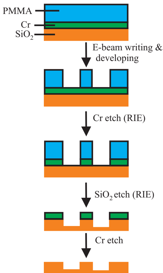
Figure 2-2 Schematic illustration of the patterning of solid substrates using electron-beam lithography and wet and/or reactive ion etching. For patterning relief structures in silicon a four-layer mask consisting of Si, S1813-resist, Ge, and PMMA was used following a similar sequence of steps as depicted here
