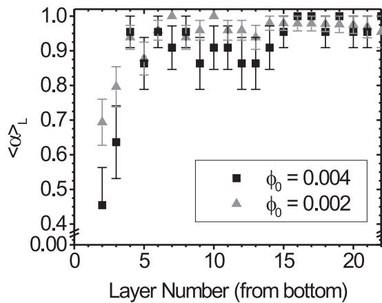
Figure 8-2 Layer-averaged stacking parameter as a function of layer number from the bottom plane of the sample for a system of 1- \mu m diameter silica colloids sedimented from volume fractions of 0.004 and 0.002.
