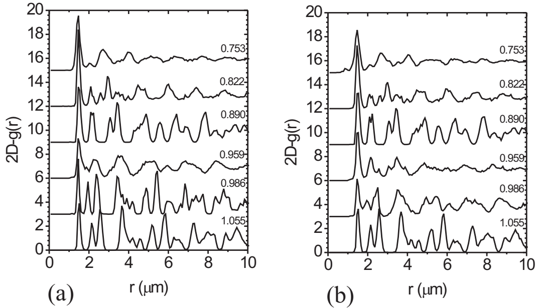
Figure 4-9 In-plane (2D) radial distribution functions for the epitaxial HCP-FCC transition (a) at the third layer from the template and (b) at the tenth layer from the template. Curves for different values of \epsilon are shifted by 3 for clarity. Values for a/a_{HS} are indicated at the right side of every curve.
