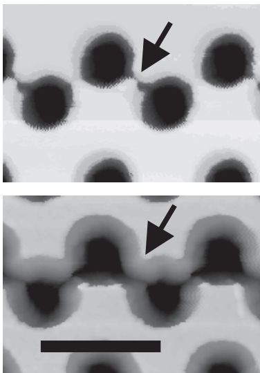
Figure 2-1 AFM images of an hcp(1100)-template in PMMA. The top figure has been written with an electron-beam dose of 135.000 \mu\text{C}/\text{cm}^2 , the figure at the bottom with a dose of 140.000 \mu\text{C}/\text{cm}^2 , the defocus has in both cases been set to 800 nm. The arrows indicate the positions where the asymmetry in the hole pattern becomes visible in an overlap between neighboring holes. The depth of the holes in the middle (dark area) is 450 nm. The length of the scalebar is 4 \mu\text{m} .
