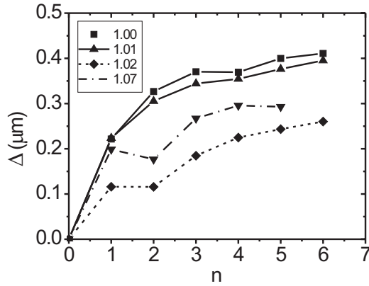
Figure 4-22 Root-mean-squared displacements with respect to the template as a function of double-layer index for the anisotropically stretched template with a/a_{HS} = 1.076 . The values in the inset give the different values of the axis ratio c/c_{HS} \cdot (a/a_{HS})^{-1} .
