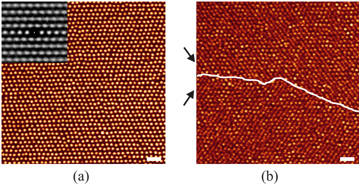
Figure 5-3 Confocal images focused (a): at a surface layer with bcc(110)-symmetry, and (b): in between the second and third layer above (a) ( a=1.60\text{ }\mu\text{m} , \phi=0.18 ). The inset in (a) shows the corresponding 2D coordinate autocorrelation graph. The arrows in (b) denote the two twinned orientations visible in the two-layer bcc(110)-projection. The white line indicates the grain boundary. The scalebars are 5\text{ }\mu\text{m} in length.
