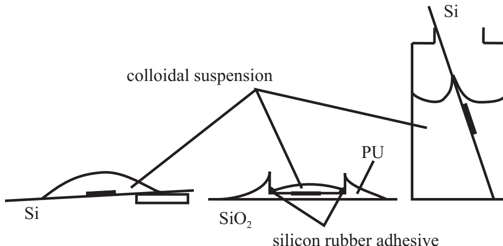
Figure 6-1 Schematic illustration of the various ways in which substrates were placed for controlled drying. The first two drawings illustrate the tilted-horizontal setup with silicon and polyurethane substrates respectively, the drawing on the right hand side illustrates the setup for vertical controlled drying. Apart from slightly tilted as in this illustration, the substrate was also placed almost completely vertical as in Figure 6-2. The thicker dark areas indicate the position of the templated area on the substrate.
