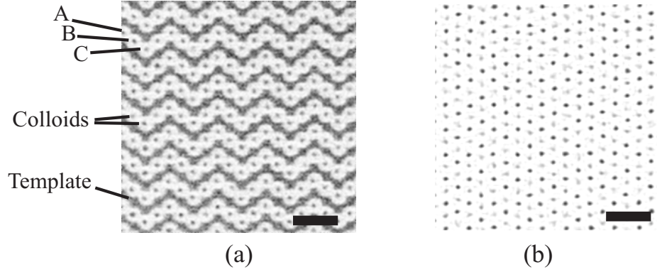
Figure 4-6 Confocal images of (a): template and particles in the first layer of a dhcp (ABCBA) crystal, and (b): the 10 th layer at a depth of 8 \mu\text{m} . The length of the scalebar is in both images 5 \mu\text{m} .
