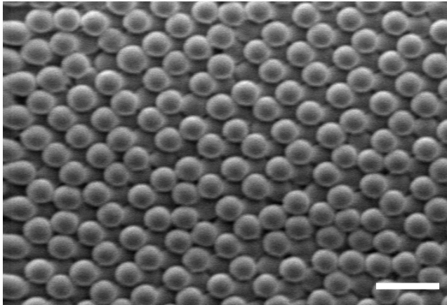
Figure 6-5 SEM image of the top layer of 870 nm-diameter colloids arranged on a poly-urethane template with an hcp(1100)-symmetry. The scalebar indicates 2 \mu\text{m} .
