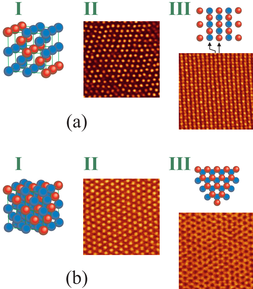
Figure 1-3 Examples of 2D confocal microscopy images (Leica TCS NT-2, 1.4 NA, 100x, excitation wavelength: 488 nm) for different crystal structures in a system with long-ranged repulsive interactions. Particles are 1.2 \mu\text{m} PMMA spheres uniformly labeled with the fluorescent dye NBD as described in [3]. (a) A low-volume fraction BCC crystal (I), together with a confocal image of the densest plane in the BCC-crystal, the (110)-plane (II). Separate particles that are completely fluorescent can still be detected due to the repulsive interaction. In a confocal image taken in between two crystal planes (III) the intensity profiles of successive planes start to overlap, which for the BCC(110)-plane leads to a striped image. (b) A high-density FCC-crystal with the same sequence (I-III) of images. In III it can be clearly seen that in between two layers separate particles can not be detected anymore.
