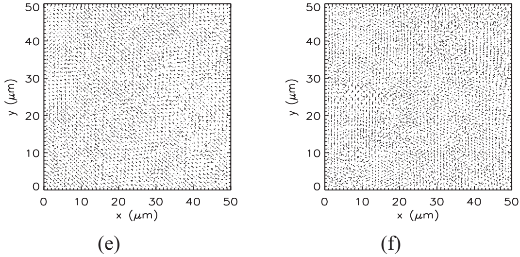
Figure 4-12 Lateral Displacements Curves (LDC's) of particles in the first twenty layers above the template. (a): a/a_{HS} = 1.055 , (b): a/a_{HS} = 0.989 , (c): a/a_{HS} = 0.959 , (d): a/a_{HS} = 0.890 , (e) a/a_{HS} = 0.822 , (f) a/a_{HS} = 0.753 . Figures (a) and (d) again correspond to 'perfect' hcp and fcc crystals respectively. In the other figures directional shifts in particle positions due to stress relaxation are visible.
