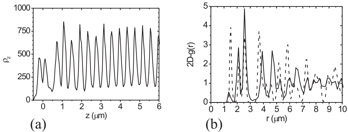
Figure 4-24 (a) Linear number density perpendicular to the template for a crystal at an anisotropically stretched template with a/a_{inc} = 1.076 and an axis ratio of c/c_{inc} \cdot (a/a_{inc})^{-1} = 1.50 .
