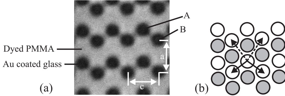
Figure 4-3. (a): Confocal microscopy image of an hcp(1100)-template, with the characteristic ABA-sequence of the close packed planes that grow perpendicular to the template indicated. The distances a and c span the 2D unit cell and their lengths are in this image 2.08 \mu\text{m} and 1.96 \mu\text{m} respectively. (b): Drawing of the projection of sphere positions in 2 successive hcp(1100)-layers. The solid arrows indicate the in-plane nearest neighbor distances r_1, r_2 ; the dashed arrows the next-nearest neighbor distances r_3, r_4 .
