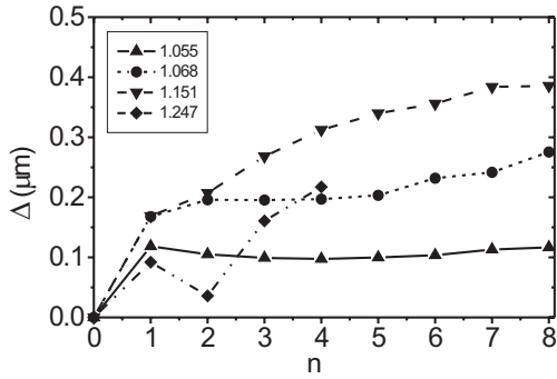
Figure 4-17 Root-mean-squared displacements of particles relative to the template as a function of double-layer index for different values of a/a_{HS} for the stretched hcp(1100)-template.
