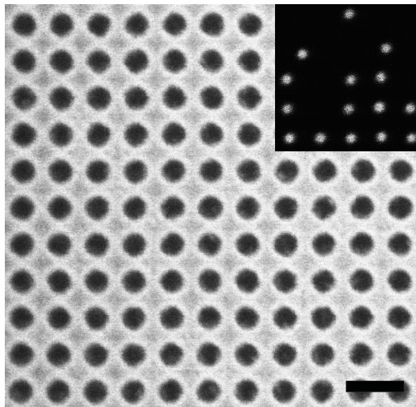
Figure 2-7 Fluorescence confocal microscopy image of a glass substrate that has been selectively patterned with the silane coupling agent-dye mixture APS-FITC (light areas) using MIMIC. The length of the scalebar is 3 \mu\text{m} . The inset shows a confocal image of 1.4 \mu\text{m} -diameter silica particles with a 400 nm-diameter core arranged on an APS-patterned template after drying from an ethanol-solution.
