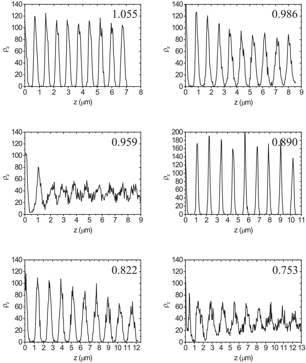
Figure 4-7 The linear number density of particles perpendicular to the hcp(1100)-template at different template-crystal mismatch. The values in the top right corners of every graph give the corresponding value for a/a_{HS} . The figures with a/a_{HS} = 1.055 and 0.890 correspond to ‘perfect’ hcp and fcc crystals respectively.
