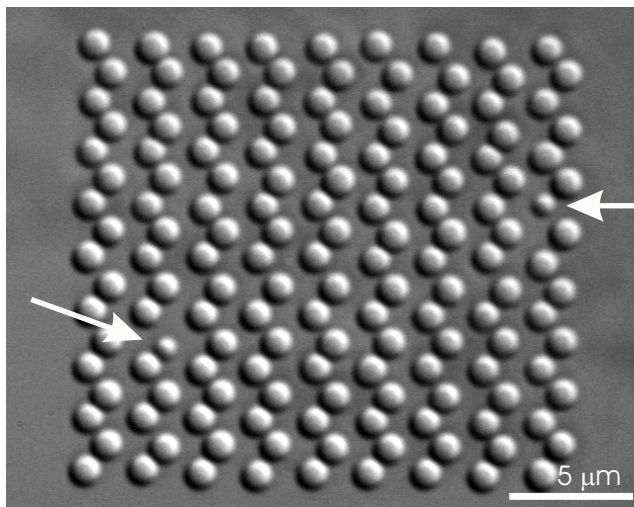
Figure 3-1: Image of a pattern of 153 1.4\ \mu\text{m} diameter silica particles arranged on a \text{hcp}(1100) lattice, taken with DIC microscopy in suspension. The arrows indicate two smaller particles that have been incorporated as defects in the pattern.
