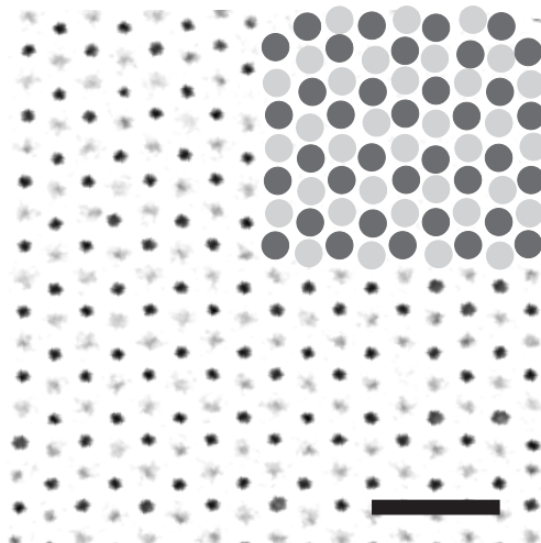
Figure 1-5 Confocal image (Leica TCS NT-2, 1.4 NA, 100x, excitation wavelength: 488 nm) taken 18 \mu\text{m} deep in a suspension containing an hcp-crystal of hard-sphere like core-shell colloids. The particles have an outer radius of 700 nm and a fluorescently (FITC) labeled silica shell with a radius of 200 nm. Particles in the next layer are vaguely visible in between the particles in focus. In the top right corner spheres have been drawn on the positions of the retrieved 3D coordinates projected in the image plane. The length of the scalebar is 5 \mu\text{m} .
