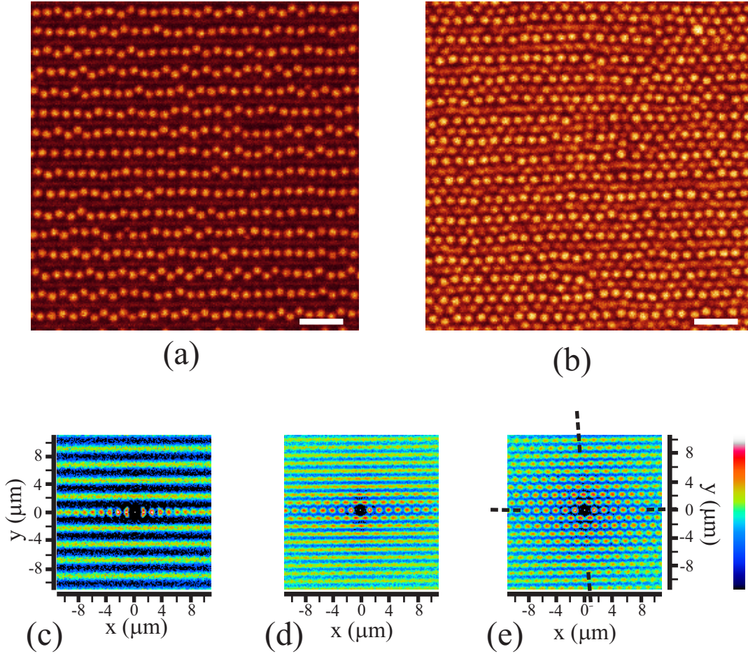
Figure 5-4 Confocal images and 2D coordinate autocorrelation graphs for a system exhibiting a 1D ordered surface plane ( a = 2.26\mu\text{m} , \phi = 0.24 ). (a) and (b) are confocal images of colloids (a): in the surface layer, and (b): at a depth of 15\mu\text{m} . The scalebars denote 5\mu\text{m} . Coordinate autocorrelation graphs are given for (c): the surface layer, (d): layer four and five with coordinates from both layers projected onto a single plane (which causes the frequency doubling compared to (a)), and (e): a depth of 15\mu\text{m} using again a two-layer projection. The color table is given on the right (blue = 0, white = 1). The dashed lines in (e) indicate the two in-plane lattice-directions.
