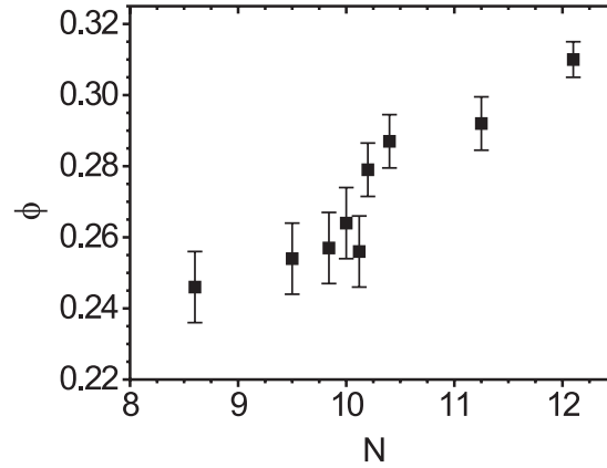
Figure 7-5 The volume fraction in the first two layers above the bottom wall as a function of sediment thickness.
