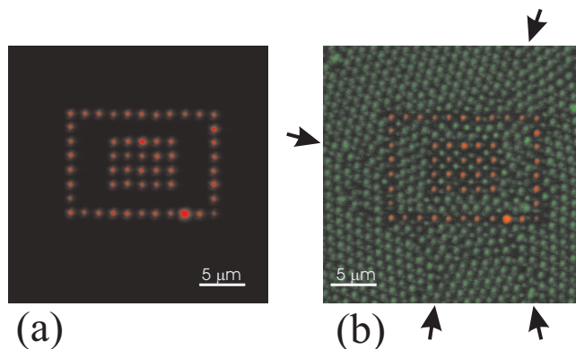
Figure 3-3 Fluorescence confocal microscopy images of (a): a pattern of 1 \mu\text{m} -diameter silica particles labeled with RITC (red), (b): after addition of FITC labeled (green) particles. The image in (b) has been taken with the focus in between the first and the second layer so that in the central square particles from both the first (red) and the second (green) layer can be seen. The arrows indicate defect-lines in the surrounding crystal originating from the patterned structure.
