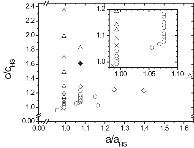
Figure 4-5 Schematic graph of crystal phases versus scaled lattice constants. The open symbols denote the occurrence of a stable phase from the template onwards: hcp ( \circ ), fcc ( \square ), or hexagonally stacked ( \Delta ); crosses (x) indicate that the structure was hcp(1100) in the third layer, while fcc(100) in the tenth layer. The filled diamond indicates a non-close packed structure. The open diamonds denote a disordered state in the first layers above the template.
