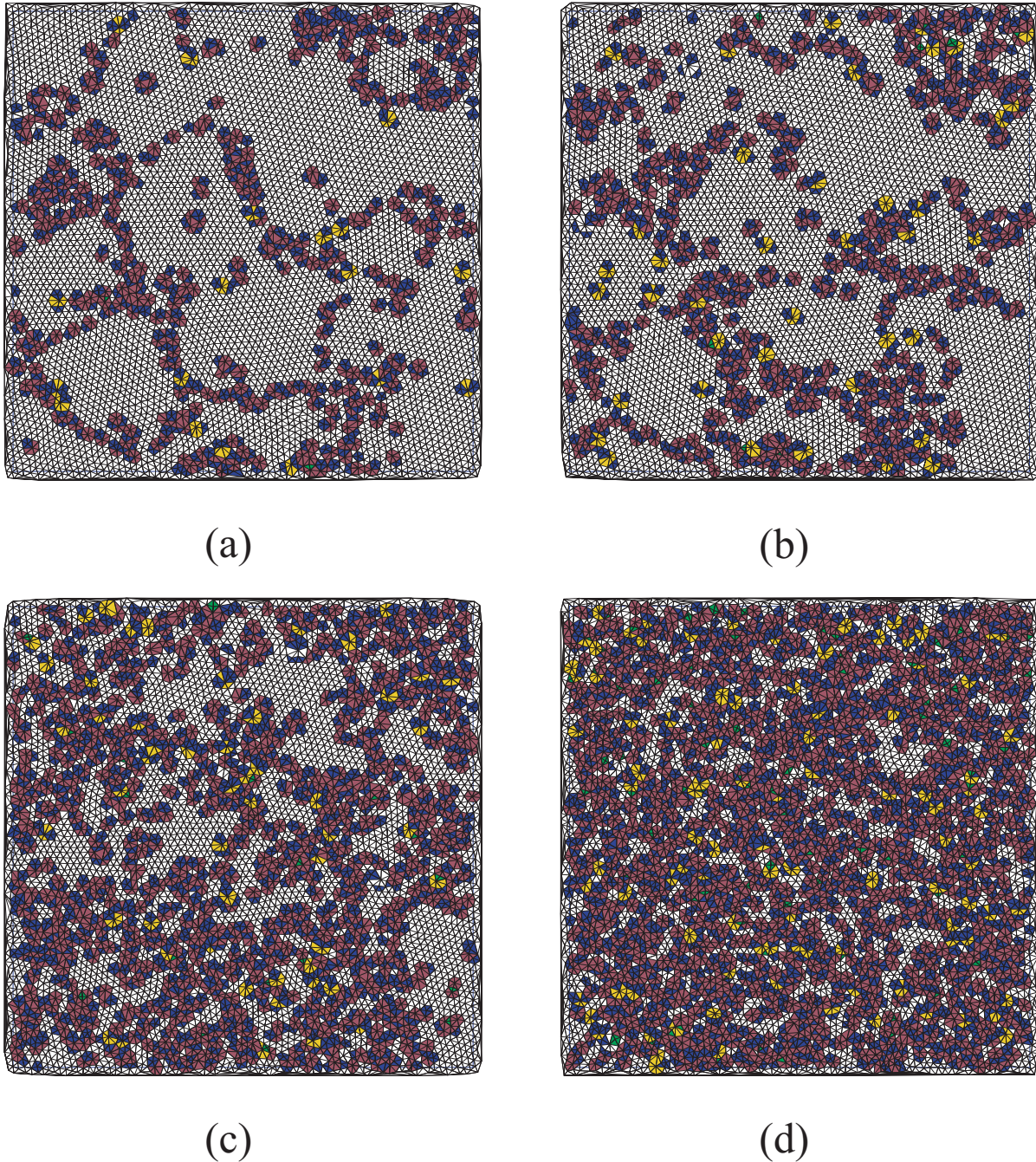
Figure 7-10 Delauney triangulations for layers (a): one, (b): two, (c): three, and (d): four at N = 10.4 . Triangles surrounding six-fold coordinated particles only have been left uncolored, while colored cells indicate a deviating coordination number: green for 4-fold, blue for 5-fold, brown for 7-fold, and yellow for 8-fold coordinated particles.
