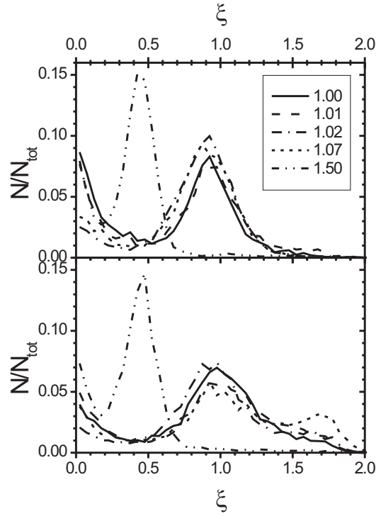
Figure 4-20 The distribution of the \xi -parameter for the anisotropically stretched template with a/a_{HS} = 1.08 . The different line types correspond to the different values of the axis-ratio, c/c_{HS} \cdot (a/a_{HS})^{-1} , as given in the inset. The lower curves correspond to the fourth layer, the upper curves to the tenth layer.
