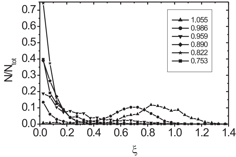
Figure 4-10 Distributions of the \xi -parameter for different values of a/a_{HS} along the HCP-FCC transition. The different symbols correspond to the different values of a/a_{HS} as given in the inset.
