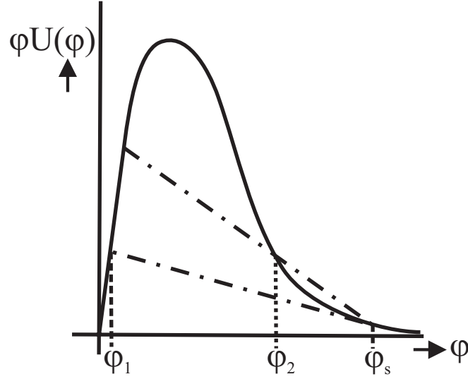
Figure 7-1 Typical form of the fluxcurve for colloidal sedimentation. \phi_s denotes the volume fraction at the top of the sediment. For initial volume fractions larger than \phi_1 a fan-region builds up starting from \phi_2 , which at continuing sedimentation expands to smaller volume fractions. For initial volume fractions smaller than \phi_1 , the sedimentation flux is constant throughout the sample until the top of the sediment.
