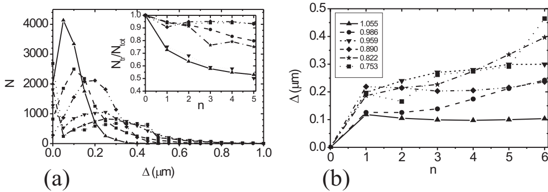
Figure 4-13 (a) Distribution of the root-mean-squared xy -displacements \Delta of particles in successive layers. The inset shows the relative number of particles contained in LDC's as a function of two-layer index n . The different lines correspond to a/a_{HS} = 1.055 (solid), 0.986 (dash), 0.959 (short dash), 0.890 (dash-dot-dot), 0.822 (dash-dot), and 0.753 (dot). (b) The averaged \Delta as a function of n . The symbols correspond to different values of a/a_{HS} as given in the inset. Lines connecting data for each a/a_{HS} have been drawn to guide the eye, where the line type for each a/a_{HS} corresponds to that in (a).
