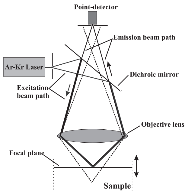
Figure 1-2 Schematic image of the operating principle of a confocal microscope. The straight lines indicate the path followed by excitation and detected emission light (assuming fluorescence microscopy). The dashed lines indicate the beam path of light generated by an out-of-focus source, which is effectively rejected by the pinhole aperture of the point-detector.
