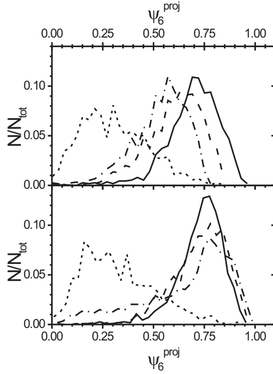
Figure 4-16 Distribution plot of \psi_6^{proj} for the stretched HCP-template for a projection of third and fourth layer (lower curves) and tenth and eleventh layer (upper curves). The different lines correspond to a/a_{HS} = 1.055 (solid), 1.068 (dash), 1.151 (dash-dot), and 1.247 (short dash).
