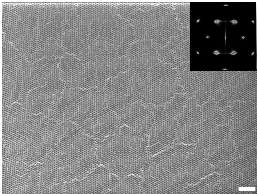
Figure 6-8 SEM image of a crystal of 870 nm-diameter particles deposited on a plain silicon substrate using vertical controlled drying. The inset shows the Fourier transform. The non-linear colortable is indicated at the right side of the inset and contains two regions of light grayscales to highlight the higher order peaks. The scalebar length is 10 \mu\text{m} .
