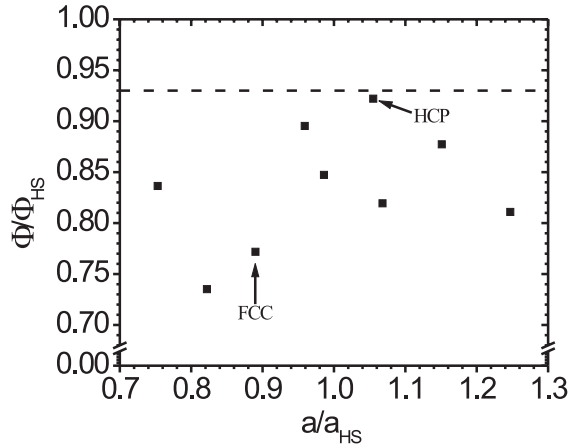
Figure 4-8 Calculated volume fractions of the epitaxially grown crystals as a function of template-crystal mismatch for the isotropically stretched hcp(1100)-template. The volume fractions have been scaled to the hard-sphere volume fraction given in Figure 4-1, averaged over the same height in the sediment as layers three to ten.
