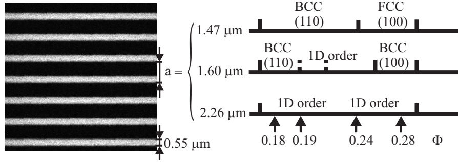
Figure 5-1 Confocal image of the striped template pattern (to the left) with the width and spacings of the lines indicated. Light areas correspond to PMMA, dark areas to 450 nm lower ITO-coated glass. For every line spacing the phase diagram of surface-layer symmetry is given. For (110)- and (100)-planes the 3D crystal structure is given as well. Phase boundaries have been indicated with an accuracy of \pm 0.02 , dashed lines indicate a coexistence region between neighboring phases. Volume fractions at which a detailed 3D structure analysis was performed are indicated at the bottom.
