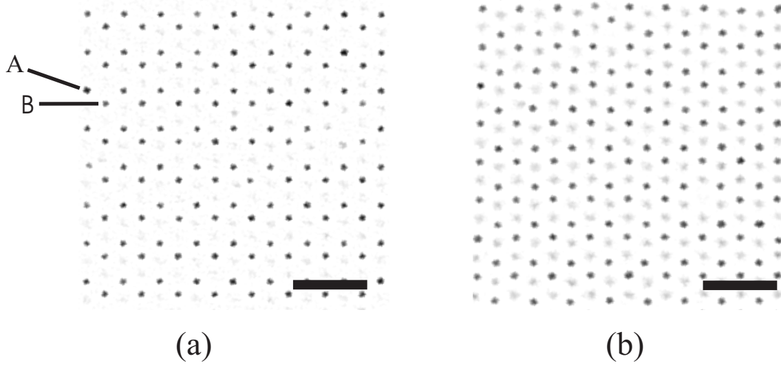
Figure 4-4 Confocal images of (a) the first layer of a templated hcp crystal and (b) the 18 th layer in the crystal, with the 19 th layer vaguely visible as well (see also Figure 1-5). Scalebars are 5 \mu\text{m} .
