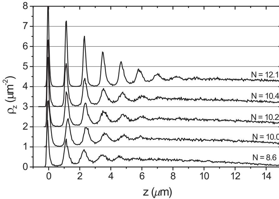
Figure 7-2 Laterally integrated density profiles as a function of sediment thickness. Profiles for different values of N have been shifted by one for clarity.
