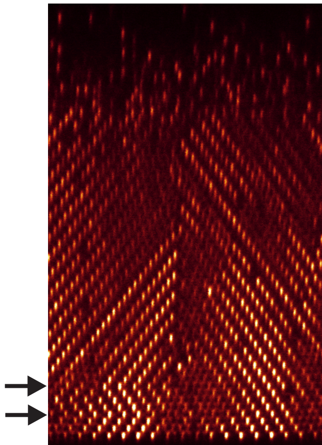
Figure 8-1 Confocal image of a (110)-plane in two adjacent grains in a sedimented crystal. The optical axis of the microscope runs in the vertical direction. The elongated shape of particle images results from the different form of the points spread function parallel and perpendicular to the optical axis. The arrows indicate two stacking faults in the left grain. At the top of the image the fluid like tail of the colloidal sediment profile is visible. The change in focus for different particles results from a small tilt of the sample with respect to the optical axis.
