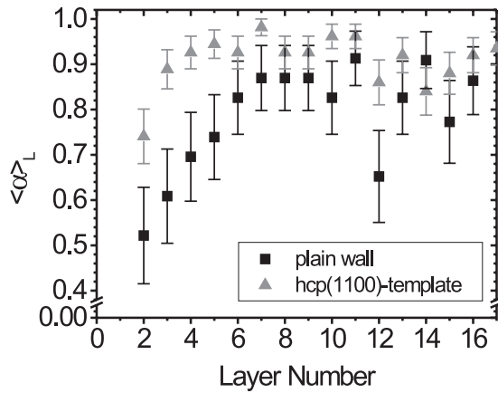
Figure 8-3 (a) Layer-averaged stacking parameter for a system of 1.4- \mu\text{m} diameter silica colloids sedimented at a plain wall (black squares) and at a mismatch hcp(1100)-template, that gives rise to a fcc(111)-surface alignment. (b) Stacking parameter as a function of grain-size for defect grains inside the otherwise monocrystalline fcc(111)-crystal at the mismatch template.
