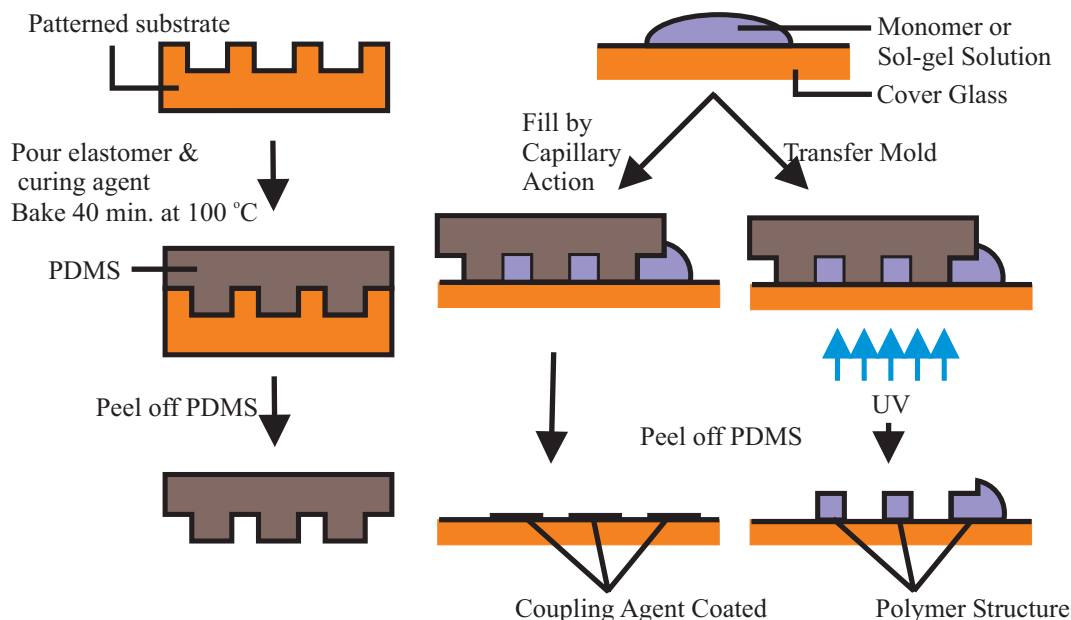
Figure 2-5 Schematic illustration of the soft-lithography techniques used in this study. The scheme to the left depicts the making of the elastomeric mold of a solid relief structure. The scheme to the right illustrates micromolding in capillaries (MIMIC) and micro-transfer molding ( \mu TM).
