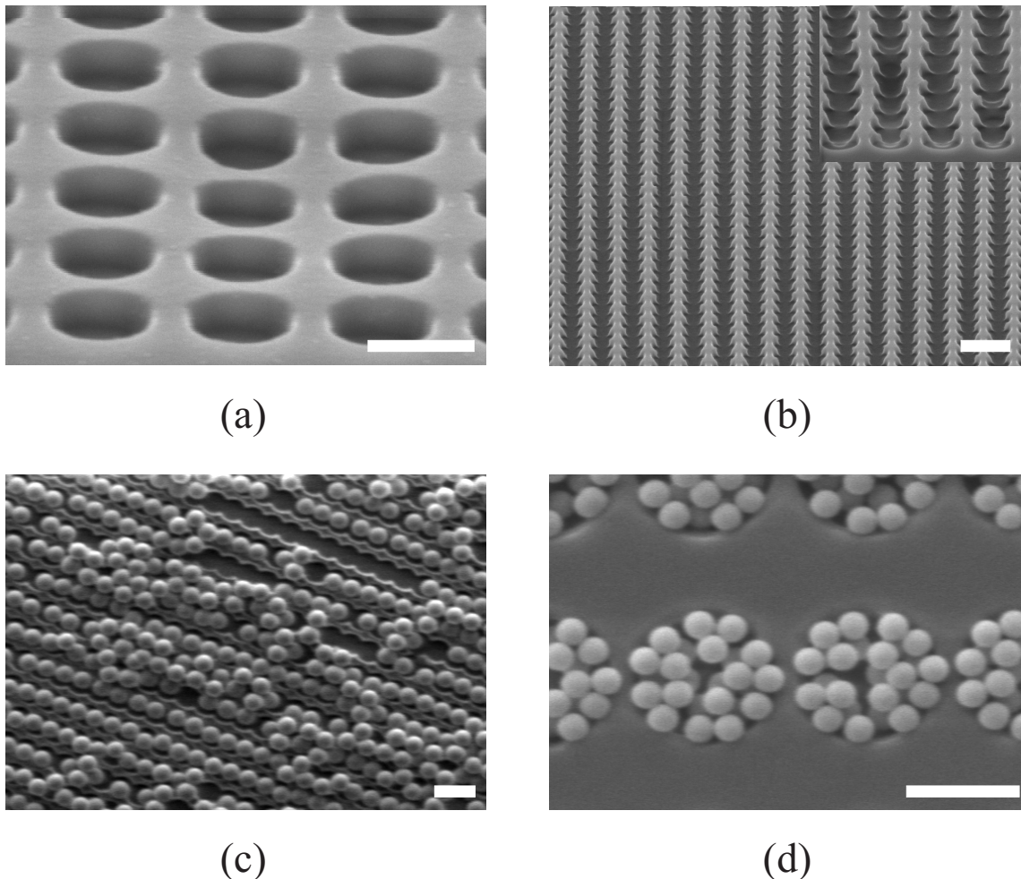
Figure 2-6 (a) and (b): SEM images of polyurethane (PU) templates made via soft-lithography. The templates consist of equally spaced rows of holes (fcc(110)-pattern). The inset in (b) shows an enlargement, where the fine reproduction of the overlap region between neighboring holes is visible. (c): 870 nm-diameter silica colloids arranged on a PU template with a 1 \mu\text{m} spacing like in (b). (d): 220 nm-diameter silica colloids that crystallized in the 1.2 \mu\text{m} -diameter holes of a PU-template in a controlled drying experiment. Scalebars are 2 \mu\text{m} in (a) and (c), and 1 \mu\text{m} in (b) and (d).
