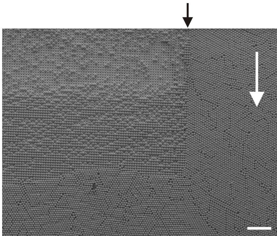
Figure 6-10 SEM image of 870 nm-diameter silica colloids arranged on a square symmetric (fcc(100)) all-silicon template after vertical controlled drying. The white arrow indicates the direction of the liquid-air interface during evaporation. The black arrow denotes the edge of the templated area. The length of the scalebar is 10 \mu\text{m} .
